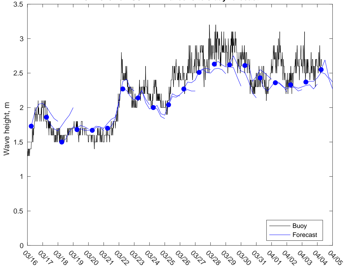
NDBC 41040 vs AUSWAV Waves: 3 to 5 day forecast
