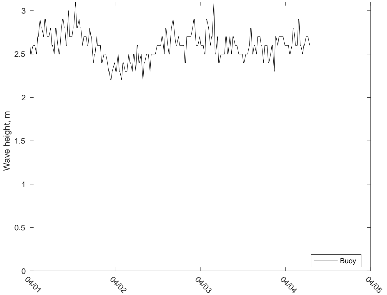
NDBC 41040 vs AUSWAV Waves: 7 to 10 day forecast
