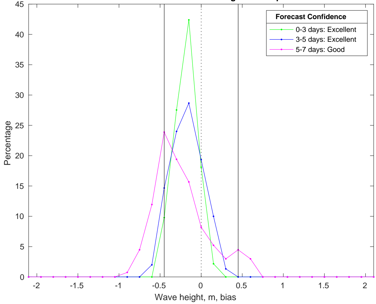
NDBC 41040 vs AUSWAV Waves Bias Histogram: 04-Apr-2025
