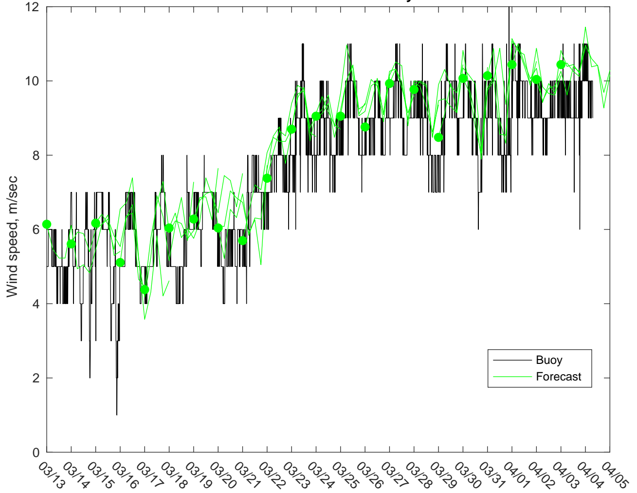
NDBC 41040 vs AUSWAV Winds: 0 to 3 day forecast
