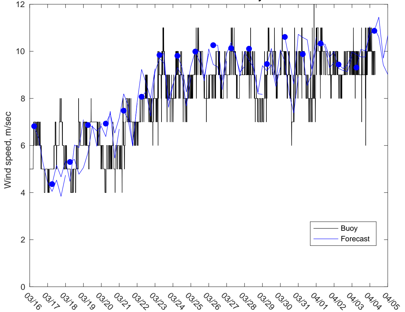
NDBC 41040 vs AUSWAV Winds: 3 to 5 day forecast
