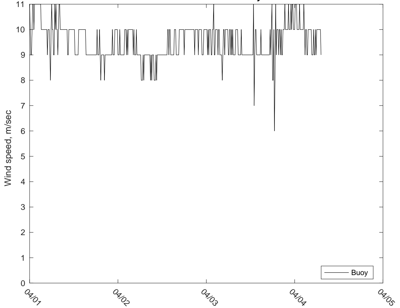
NDBC 41040 vs AUSWAV Winds: 7 to 10 day forecast
