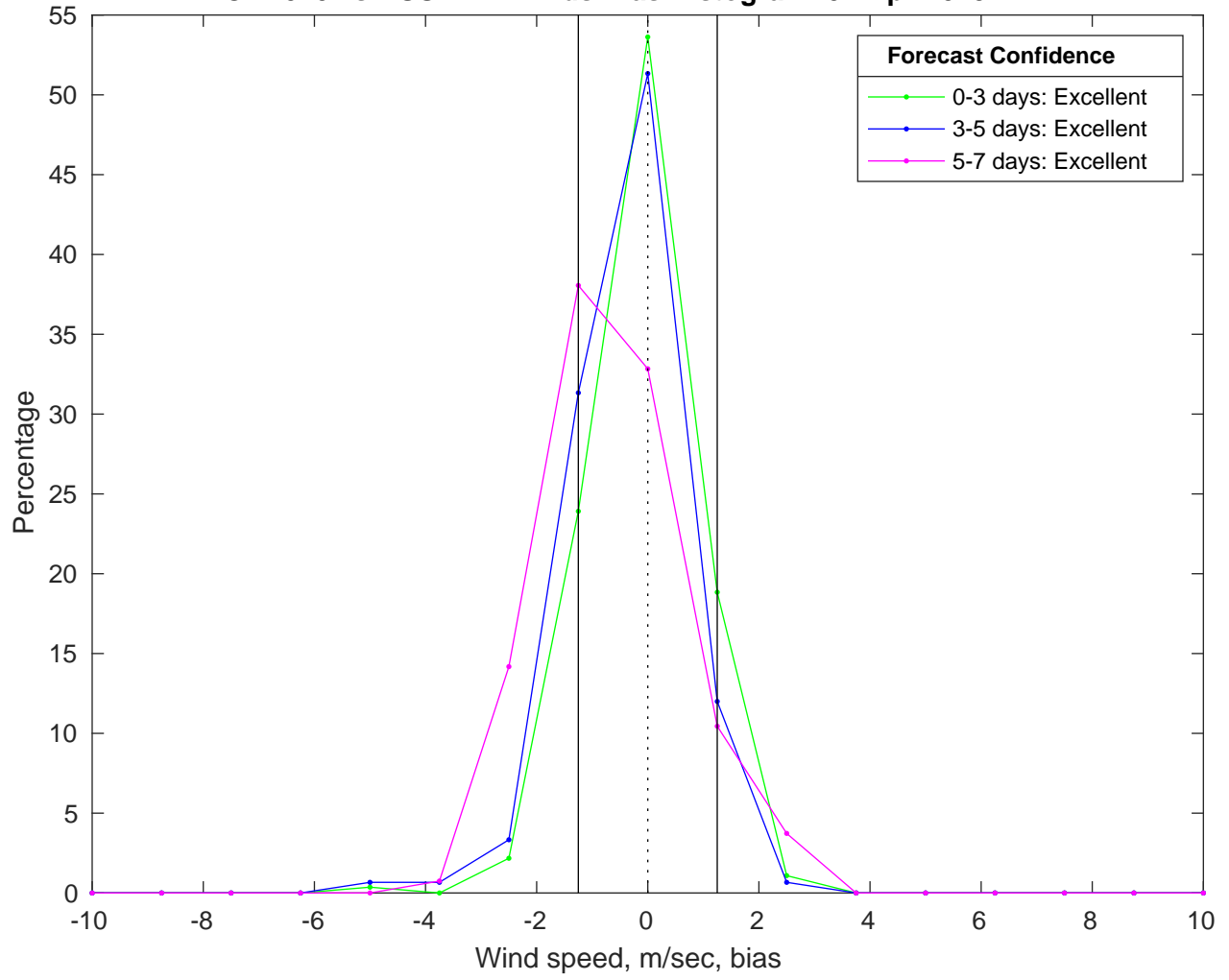
NDBC 41040 vs AUSWAV Winds Bias Histogram: 04-Apr-2025
