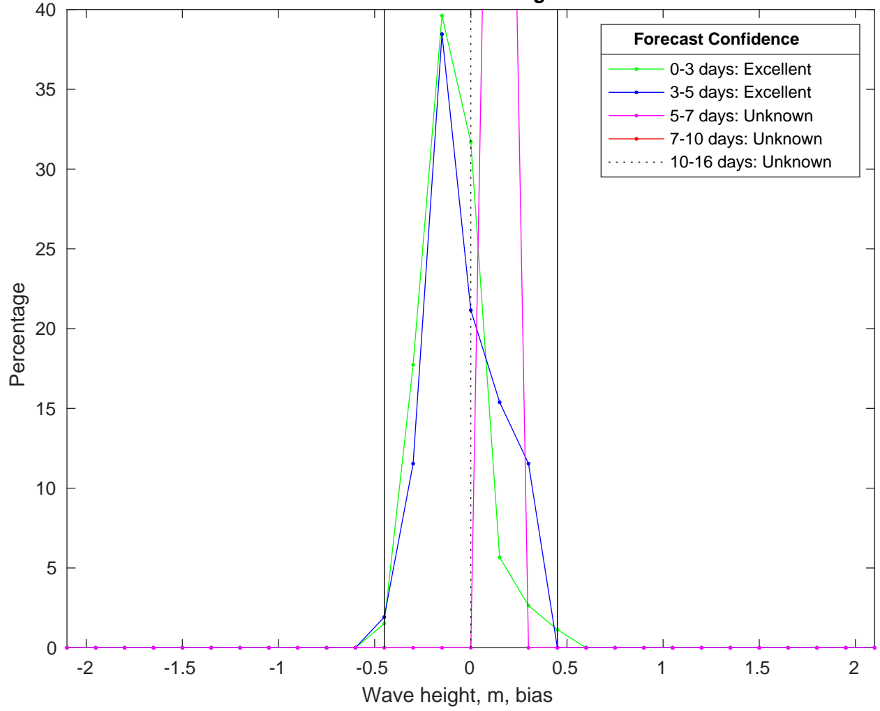
NDBC 41040 vs CMEMSWaves Bias Histogram: 18-Jan-2025
