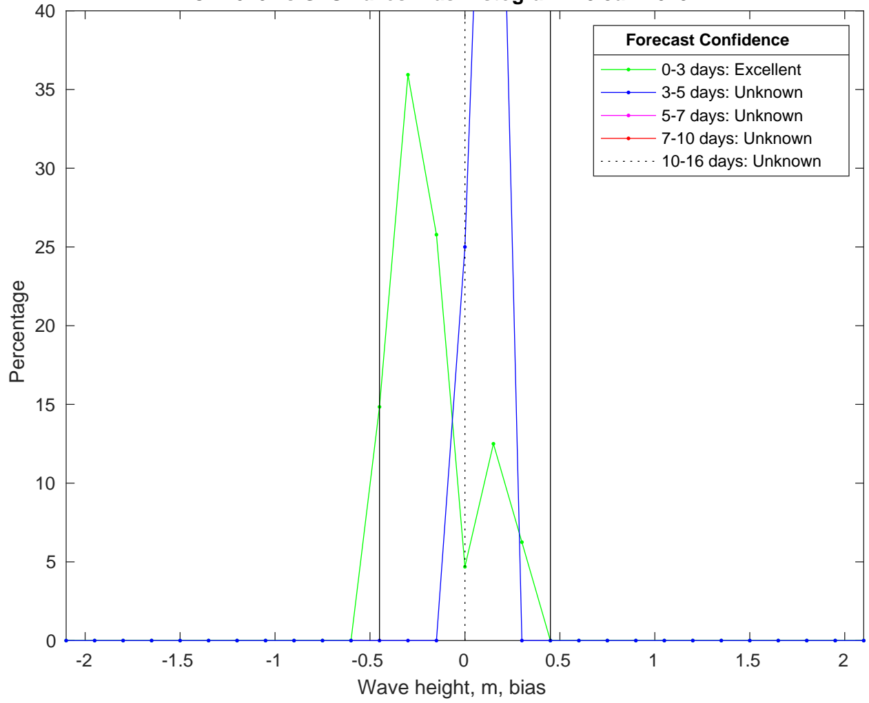
NDBC 41040 vs GFSWaves Bias Histogram: 18-Jan-2025
