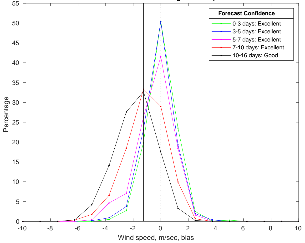
NDBC 41040 vs GFS Winds Bias Histogram: 04-Apr-2025
