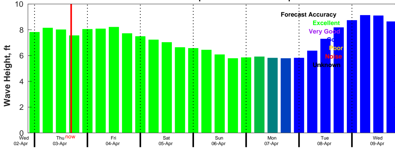
AUSWAV Wave Forecast for NDBC 41040 from 02-Apr-2025 21:00:00 to 09-Apr-2025 21:00:00
