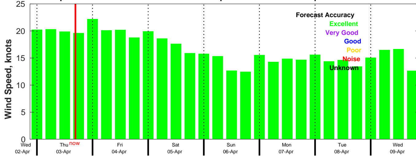
AUSWAV Wind Speed Forecast for NDBC 41040 from 02-Apr-2025 21:00:00 to 09-Apr-2025 21:00:00
