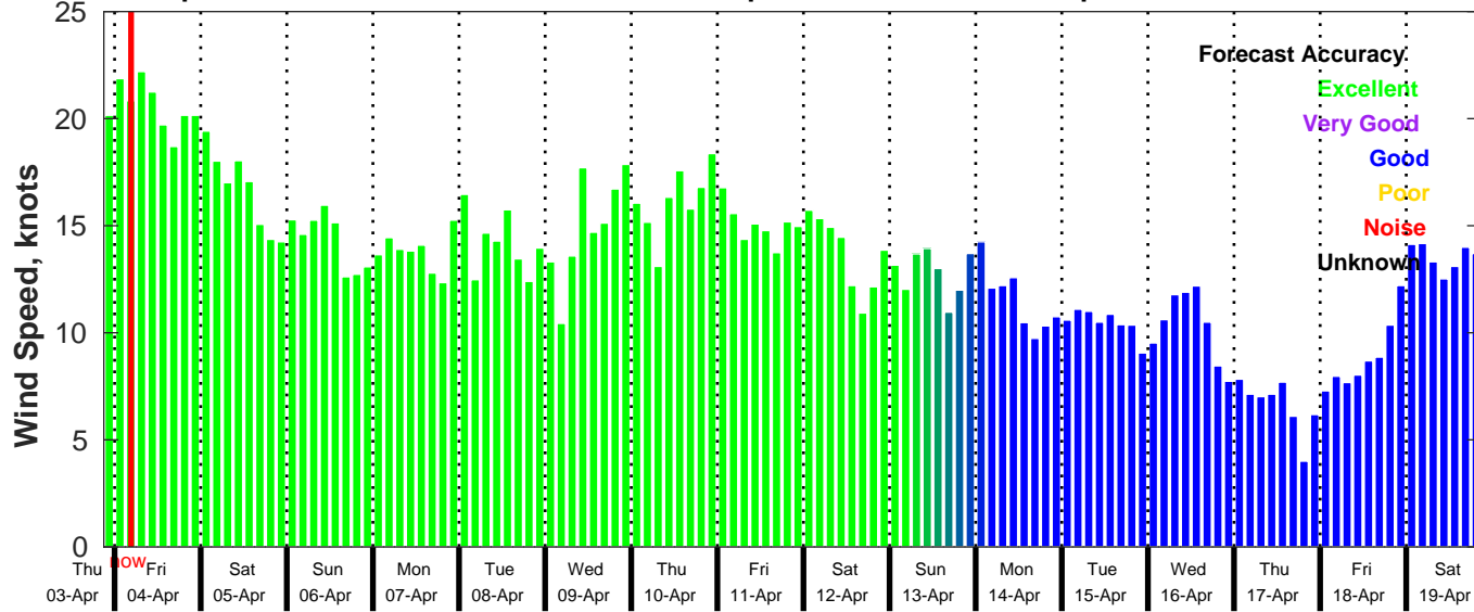
GFS Wind Speed Forecast for NDBC 41040 from 03-Apr-2025 21:00:00 to 19-Apr-2025 21:00:00
