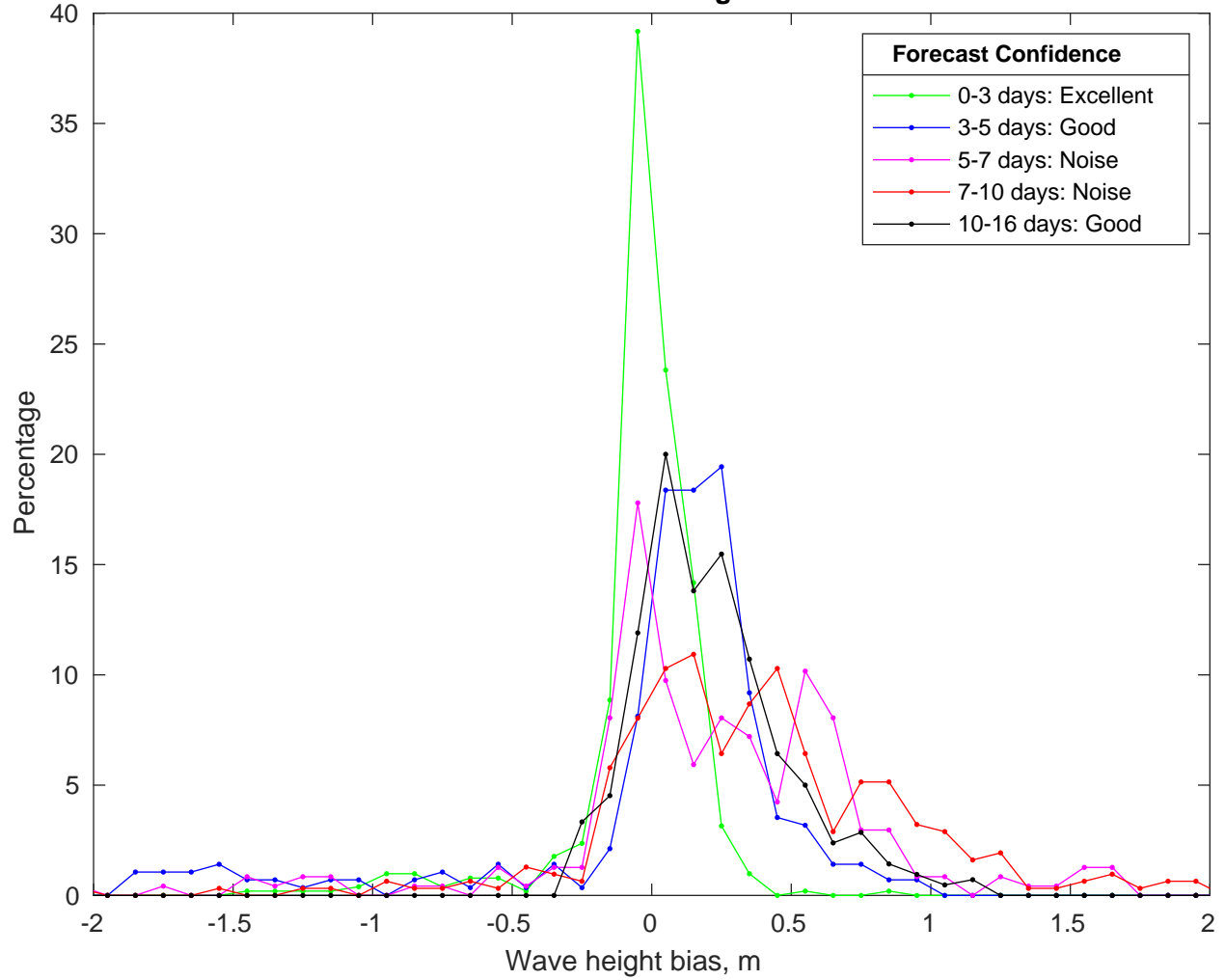
NDBC 42002 vs GFSWave Bias Histogram: 20-Jul-2024
