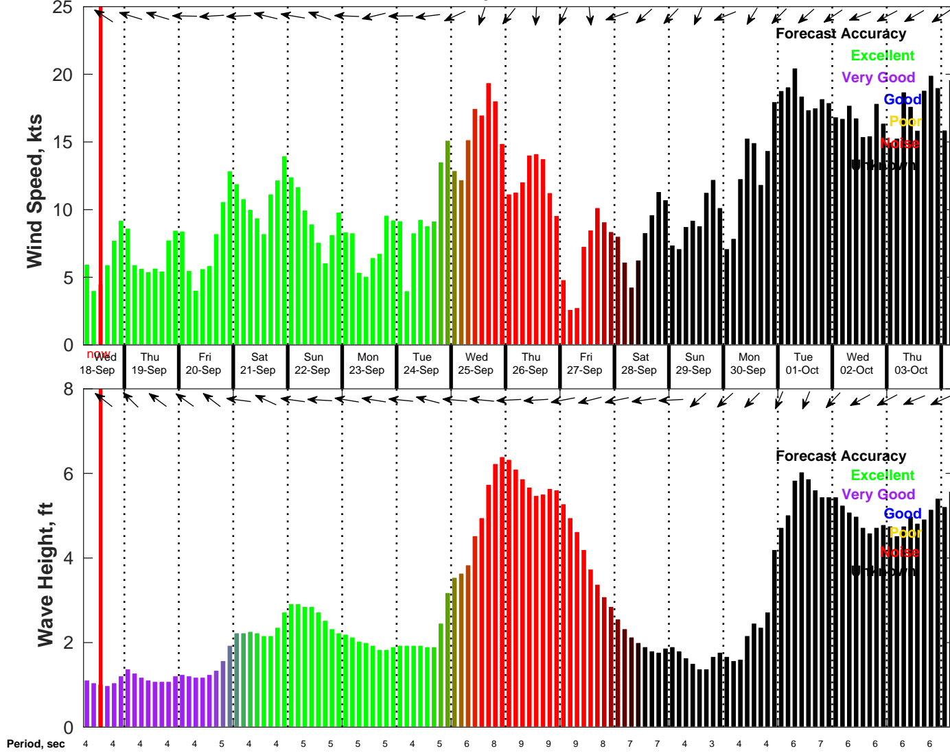
Wind & Wave Forecast for NDBC 42002 from 18-Sep-2024 06:00:00 to 04-Oct-2024 06:00:00
