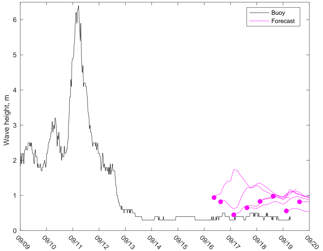
NDBC 42002 vs GFSWaves: 7 to 10 day forecast
