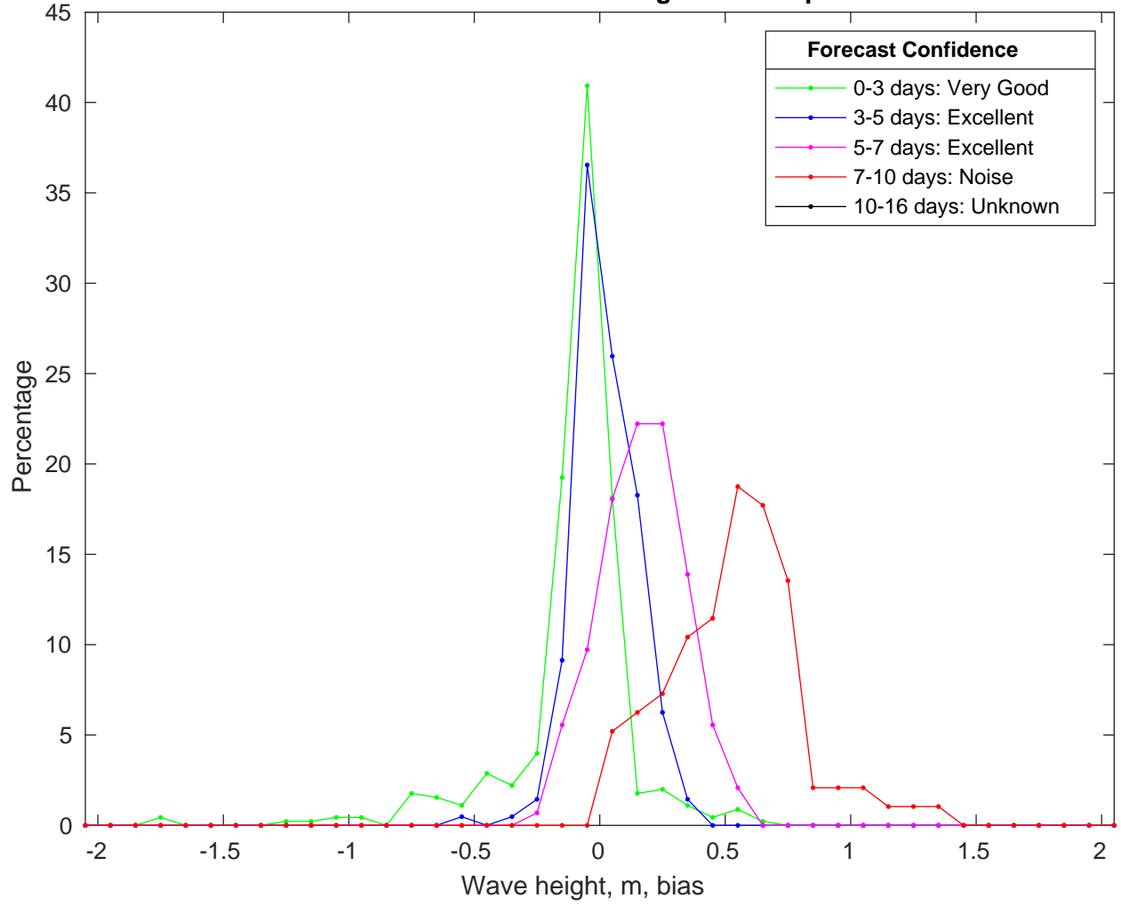
NDBC 42002 vs GFSWaves Bias Histogram: 19-Sep-2024
