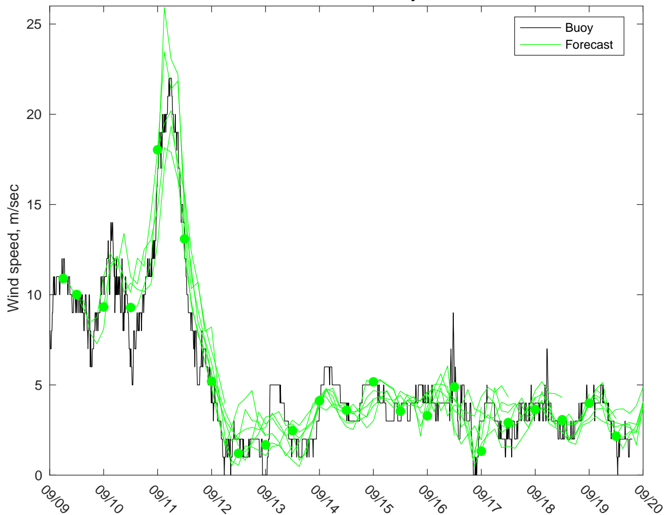
NDBC 42002 vs GFSWinds: 0 to 3 day forecast
