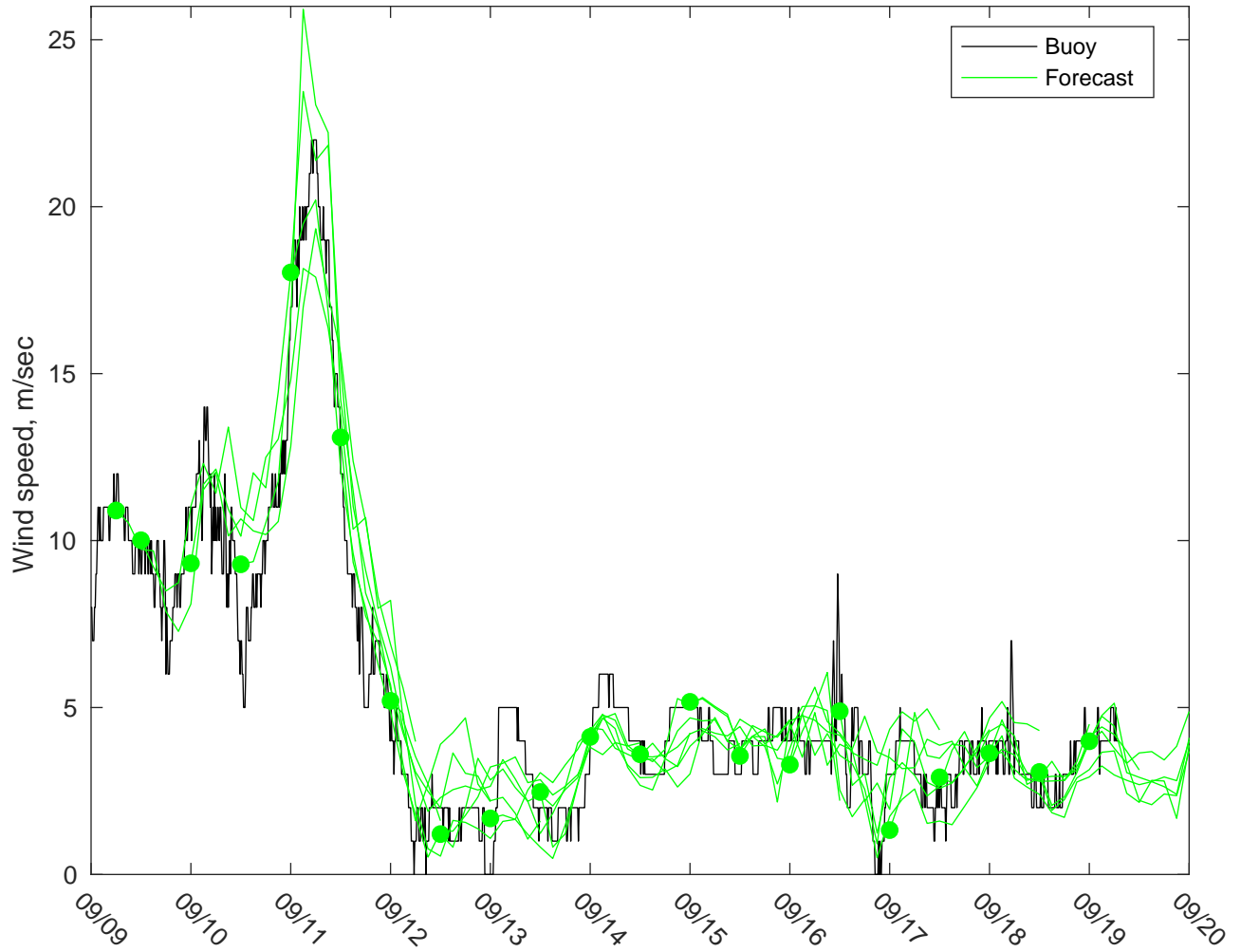
NDBC 42002 vs GFSWinds: 0 to 3 day forecast
