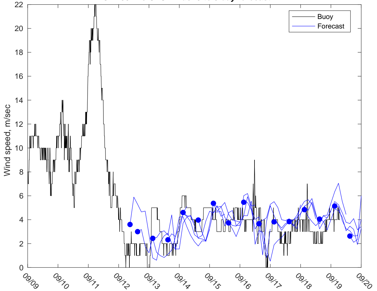
NDBC 42002 vs GFSWinds: 3 to 5 day forecast
