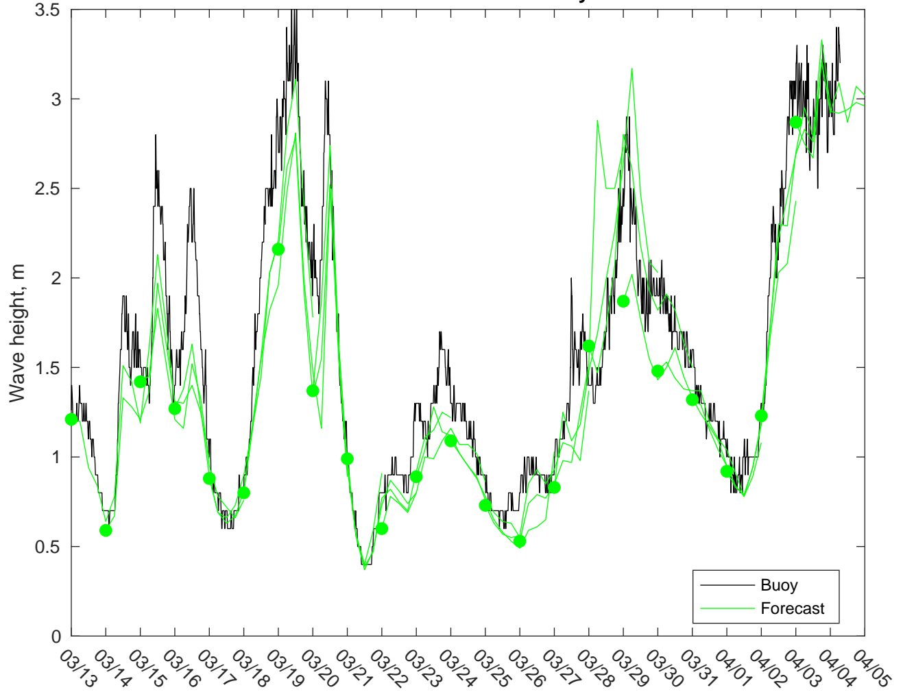
NDBC 42019 vs AUSWAV Waves: 0 to 3 day forecast
