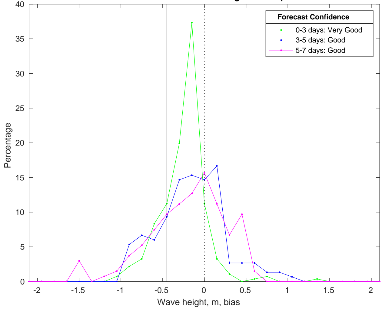
NDBC 42019 vs AUSWAV Waves Bias Histogram: 04-Apr-2025
