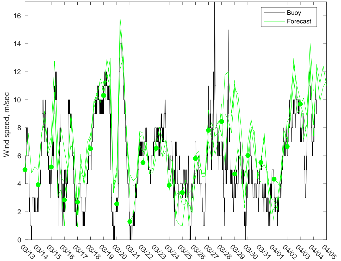
NDBC 42019 vs AUSWAV Winds: 0 to 3 day forecast
