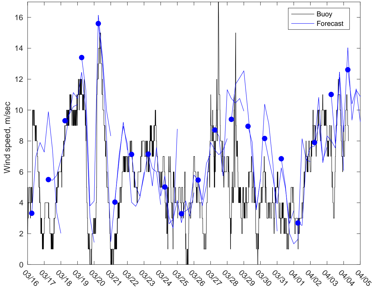
NDBC 42019 vs AUSWAV Winds: 3 to 5 day forecast
