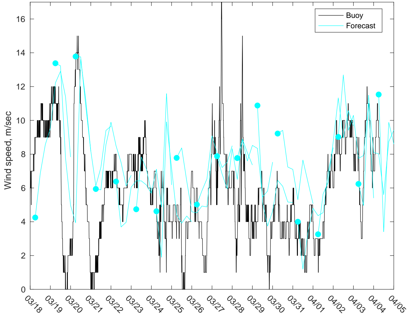
NDBC 42019 vs AUSWAV Winds: 5 to 7 day forecast
