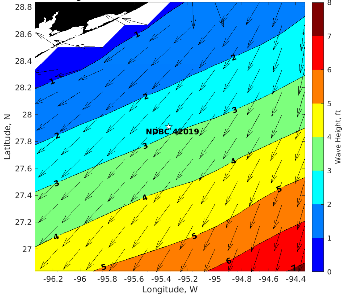
Wave Height (ft) for NDBC 42019 at 12-Dec-2024 00:00:00
