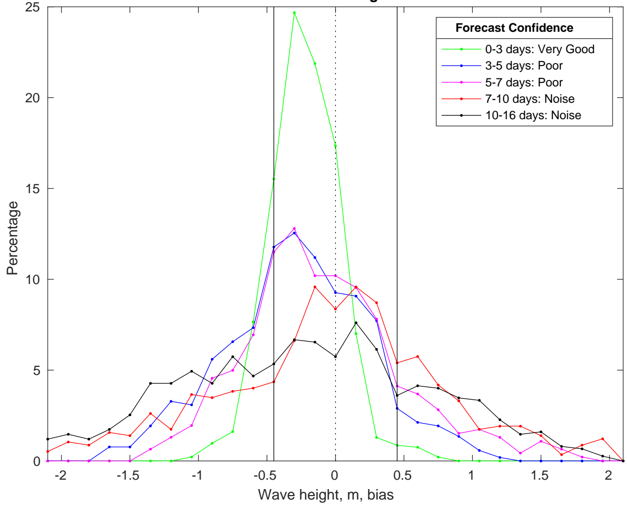
NDBC 42019 vs GFSWaves Bias Histogram: 18-Jan-2025
