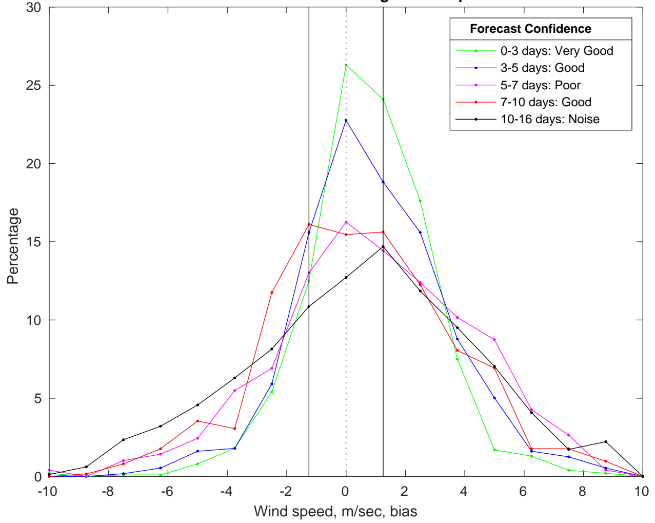
NDBC 42019 vs GFS Winds Bias Histogram: 04-Apr-2025
