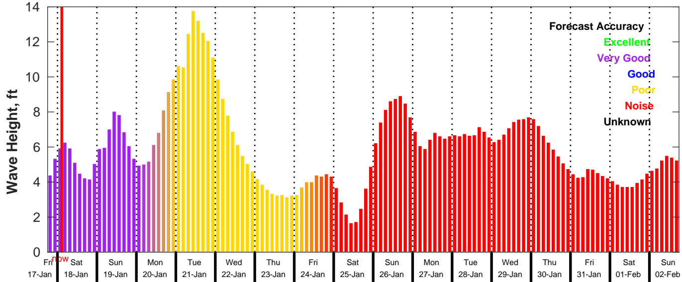
GFS Wave Forecast for NDBC 42019 from 17-Jan-2025 18:00:00 to 02-Feb-2025 18:00:00
