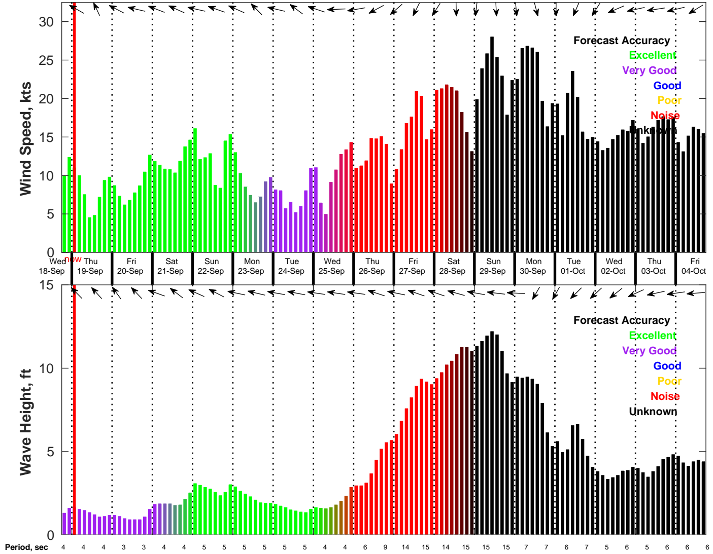
Wind & Wave Forecast for NDBC 42019 from 18-Sep-2024 18:00:00 to 04-Oct-2024 18:00:00
