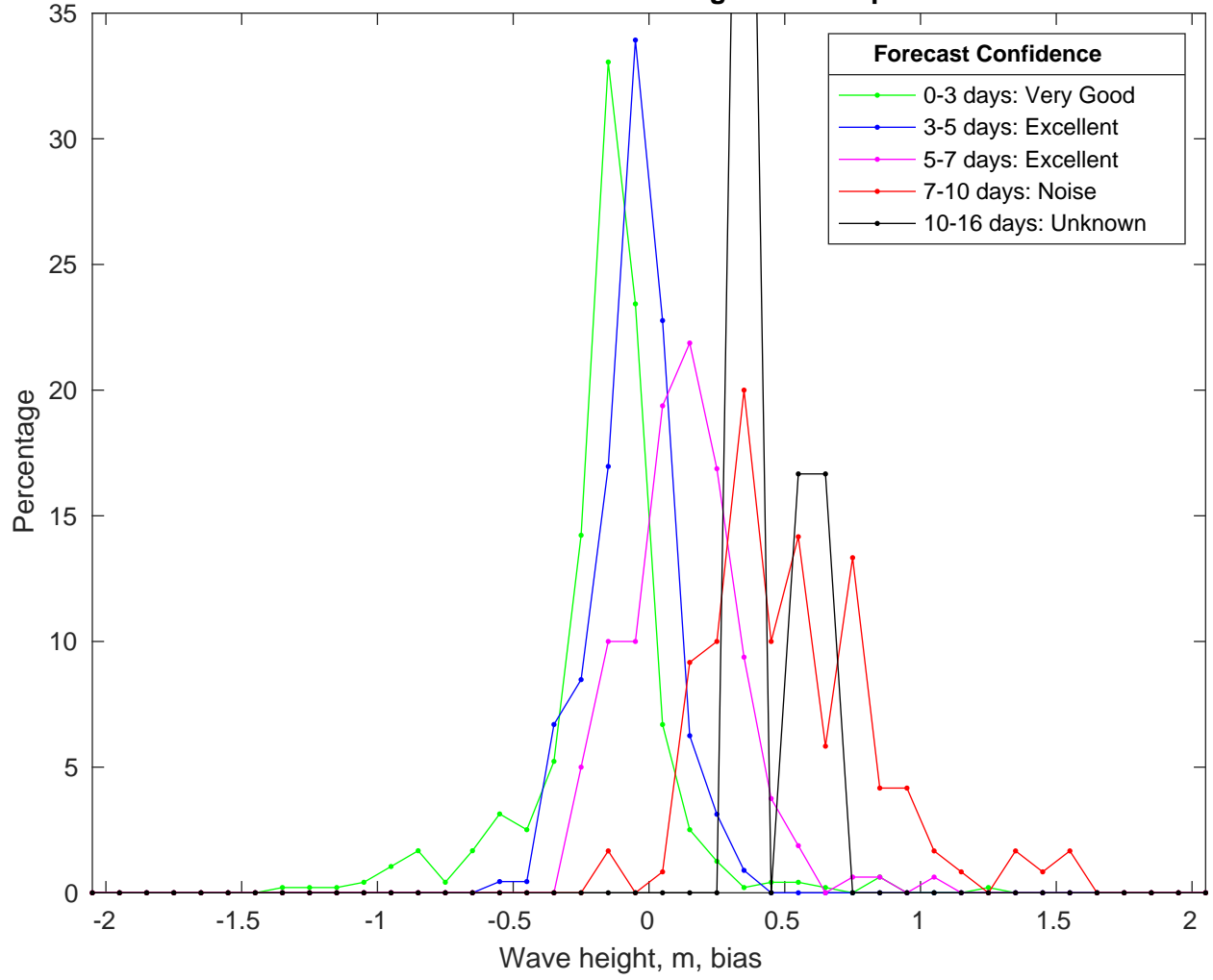
NDBC 42019 vs GFSWaves Bias Histogram: 19-Sep-2024
