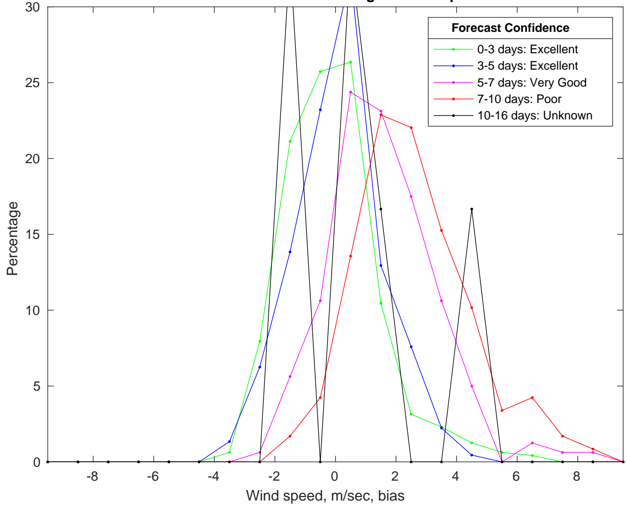
NDBC 42019 vs GFSWinds Bias Histogram: 19-Sep-2024
