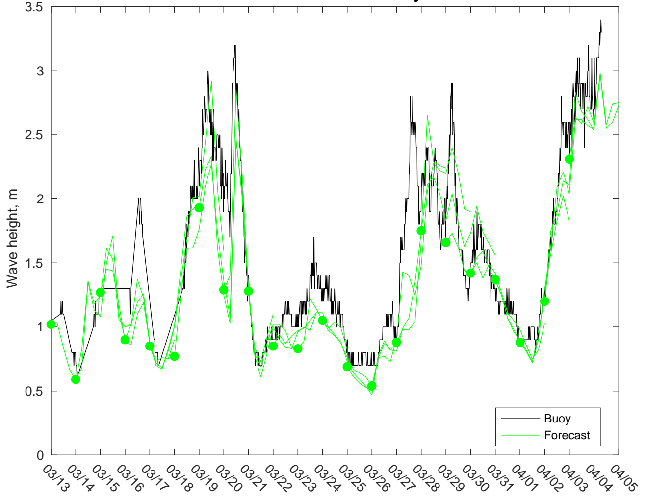
NDBC 42020 vs AUSWAV Waves: 0 to 3 day forecast
