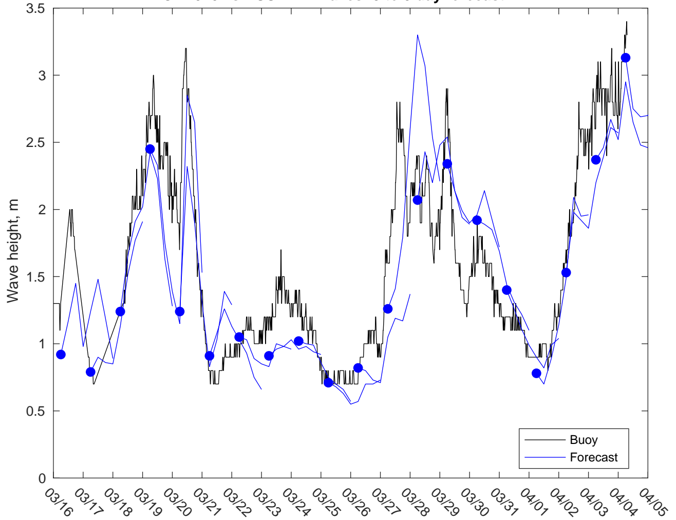
NDBC 42020 vs AUSWAV Waves: 3 to 5 day forecast
