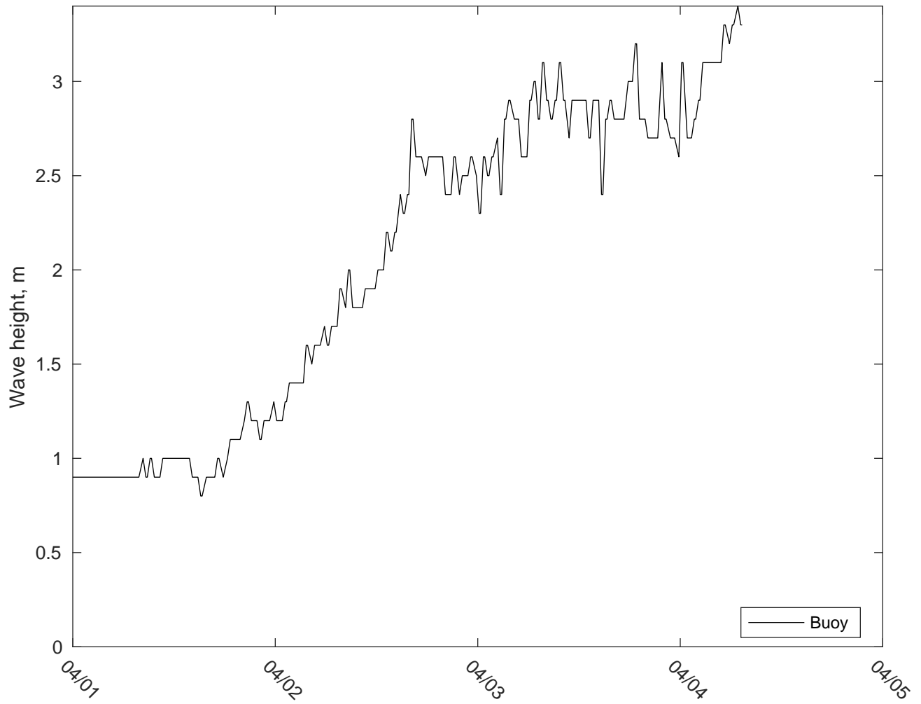
NDBC 42020 vs AUSWAV Waves: 7 to 10 day forecast
