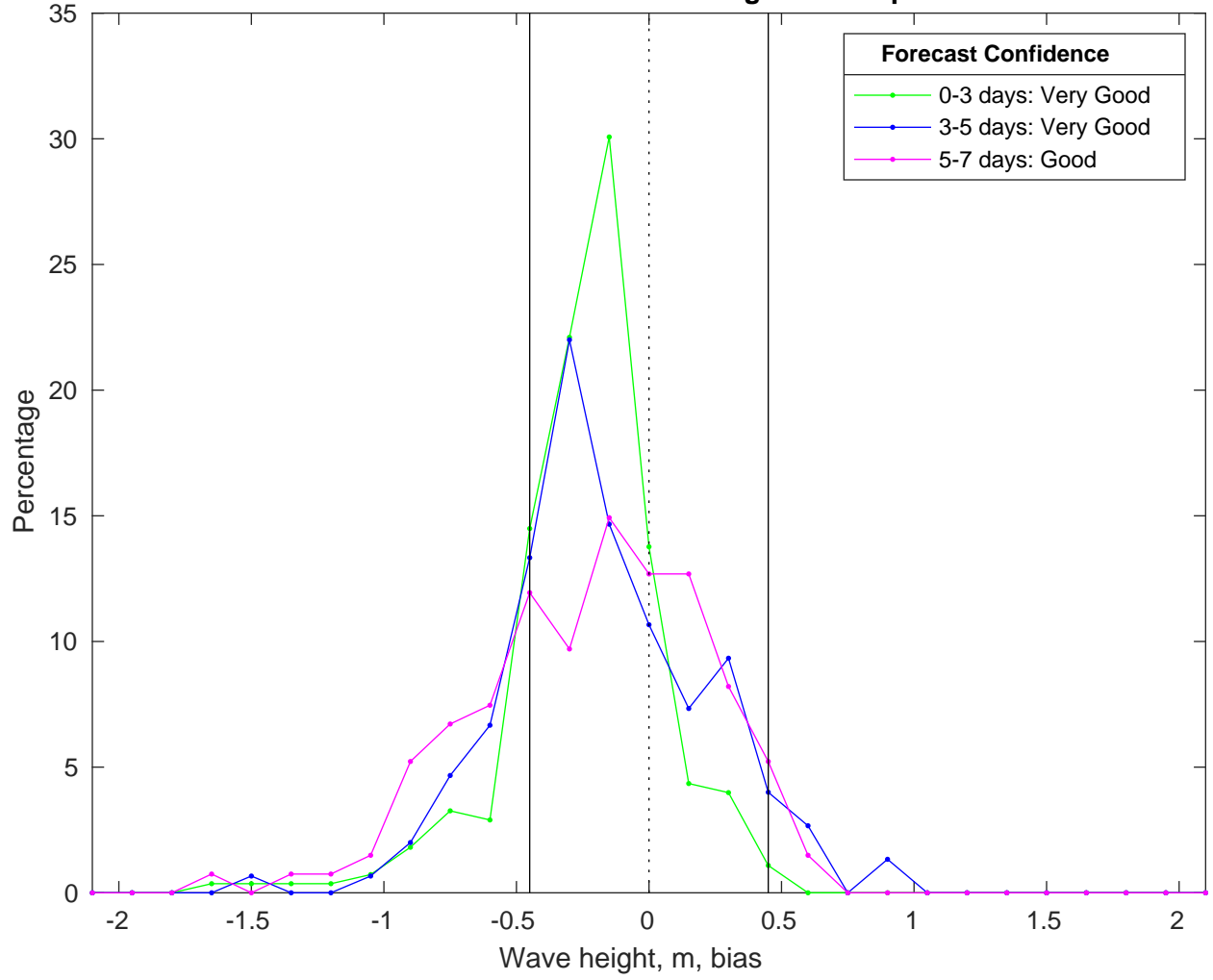
NDBC 42020 vs AUSWAV Waves Bias Histogram: 04-Apr-2025
