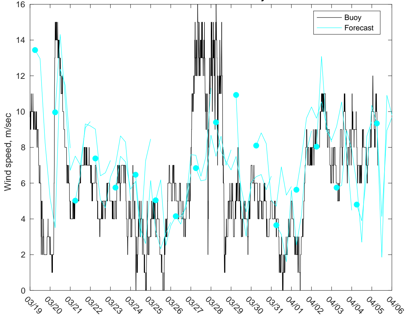
NDBC 42020 vs AUSWAV Winds: 5 to 7 day forecast
