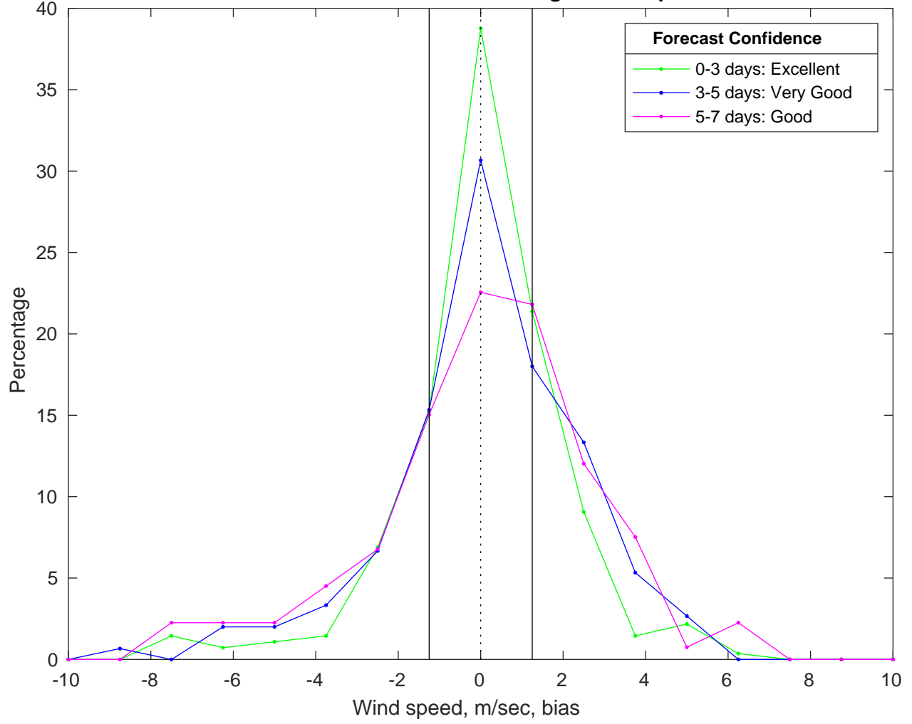
NDBC 42020 vs AUSWAV Winds Bias Histogram: 05-Apr-2025
