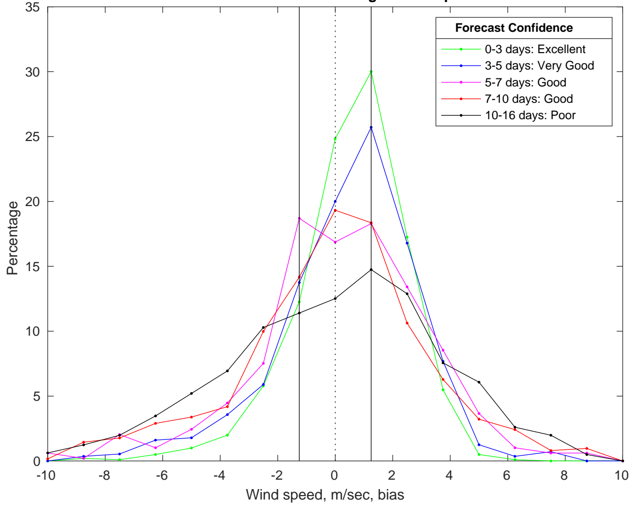
NDBC 42020 vs GFS Winds Bias Histogram: 04-Apr-2025
