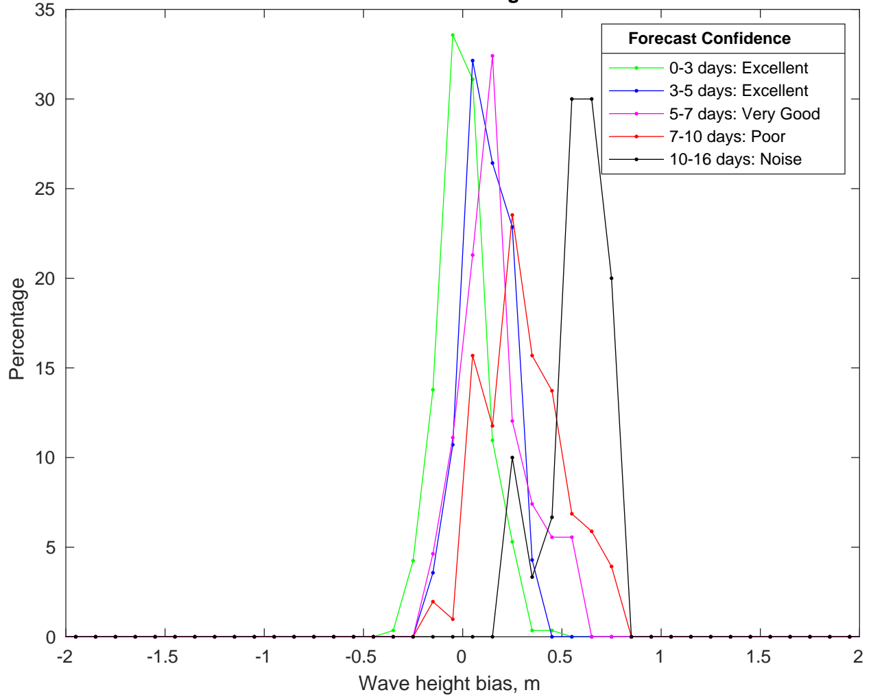
NDBC 42020 vs GFSWave Bias Histogram: 20-Jul-2024
