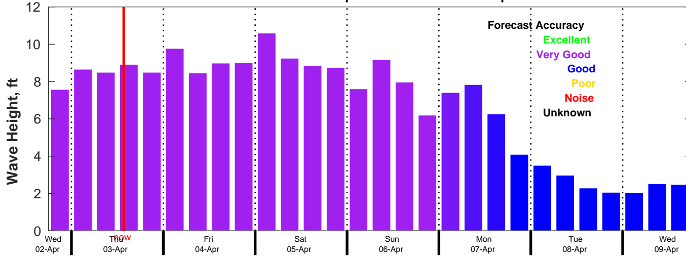
AUSWAV Wave Forecast for NDBC 42020 from 02-Apr-2025 18:00:00 to 09-Apr-2025 18:00:00
