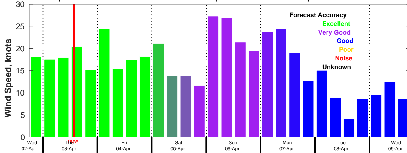
AUSWAV Wind Speed Forecast for NDBC 42020 from 02-Apr-2025 18:00:00 to 09-Apr-2025 18:00:00
