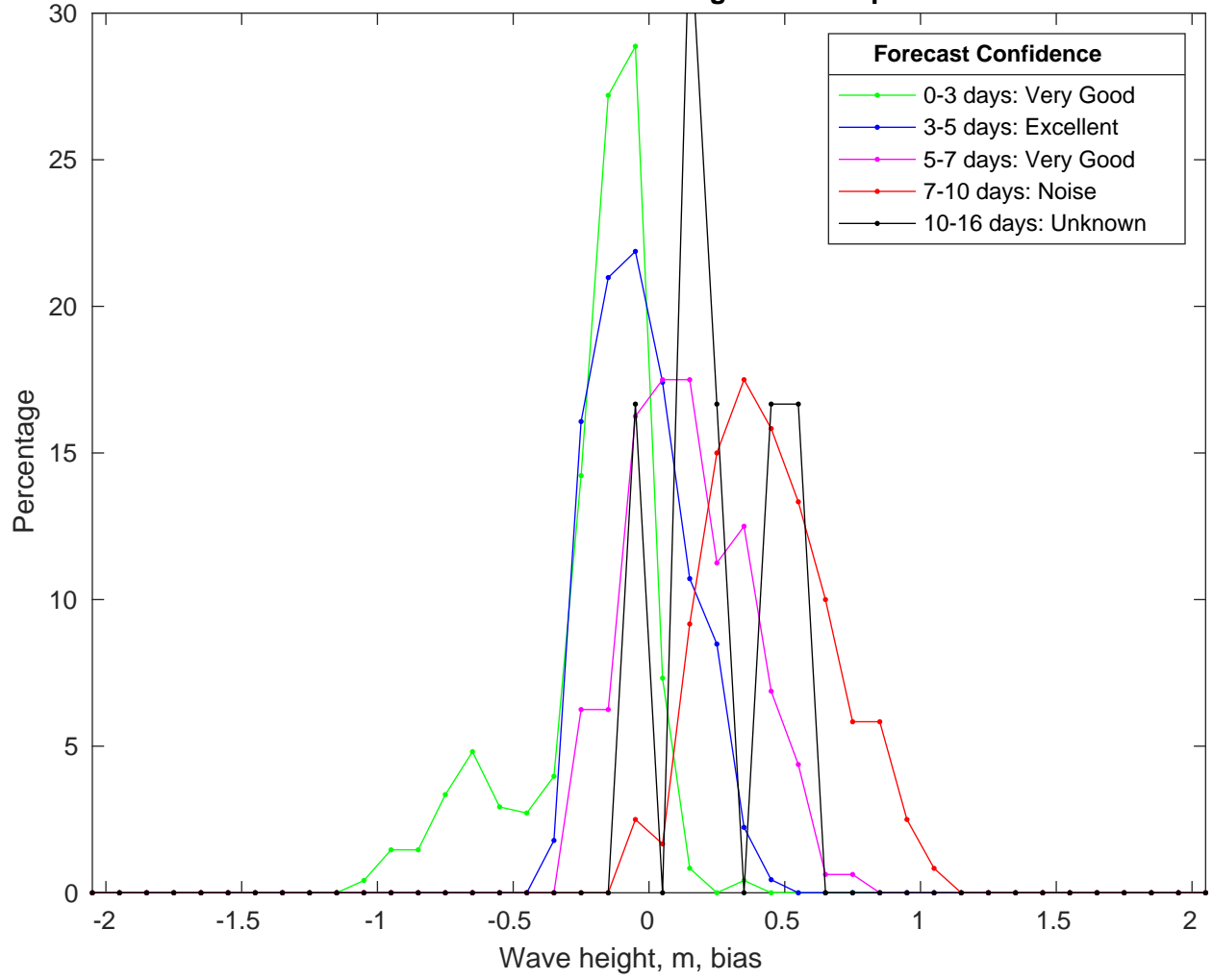
NDBC 42020 vs GFSWaves Bias Histogram: 19-Sep-2024
