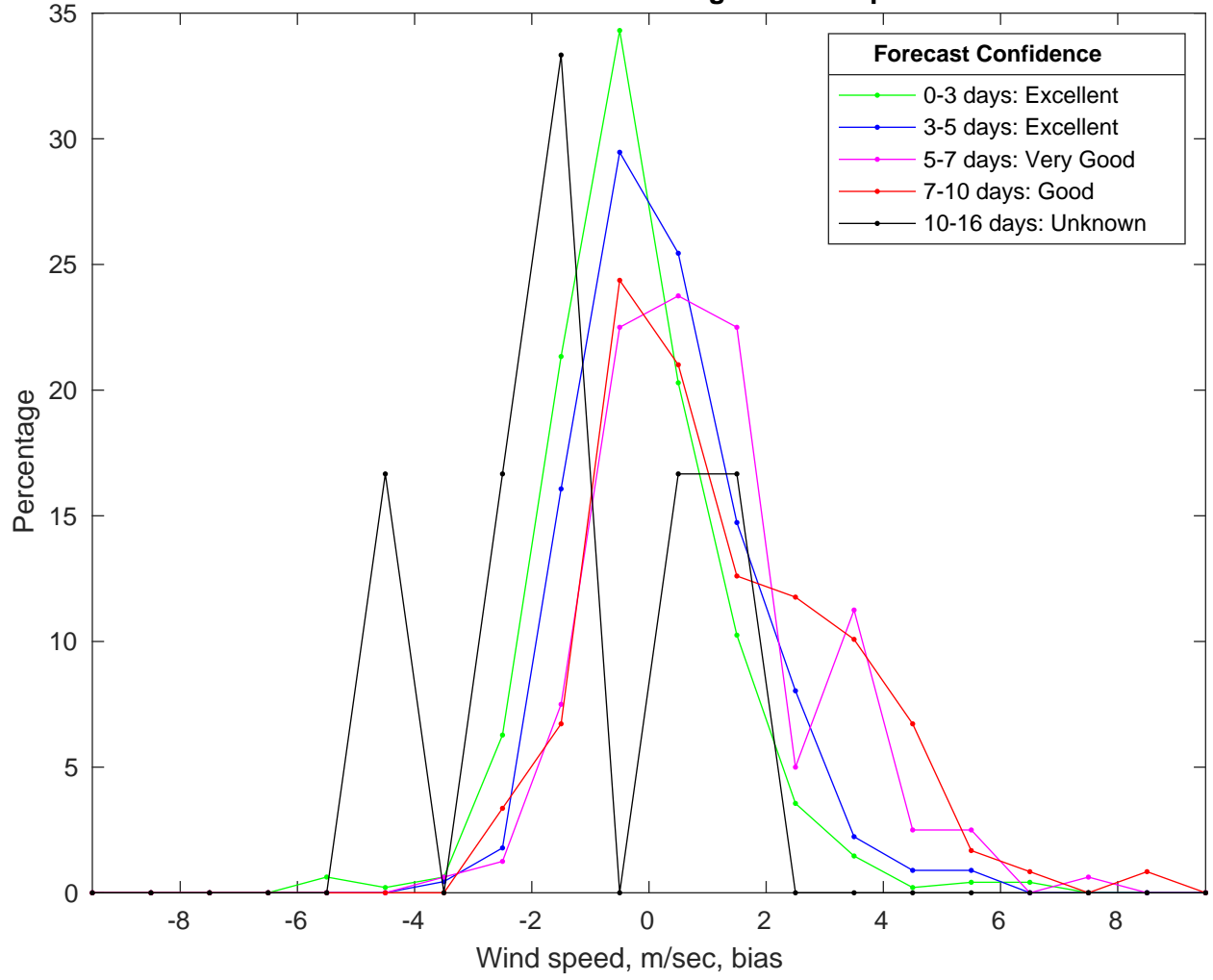
NDBC 42020 vs GFS Winds Bias Histogram: 19-Sep-2024
