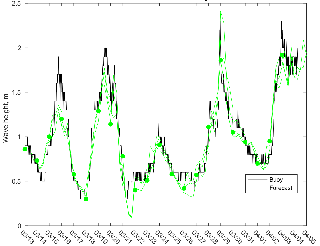
NDBC 42035 vs AUSWAV Waves: 0 to 3 day forecast
