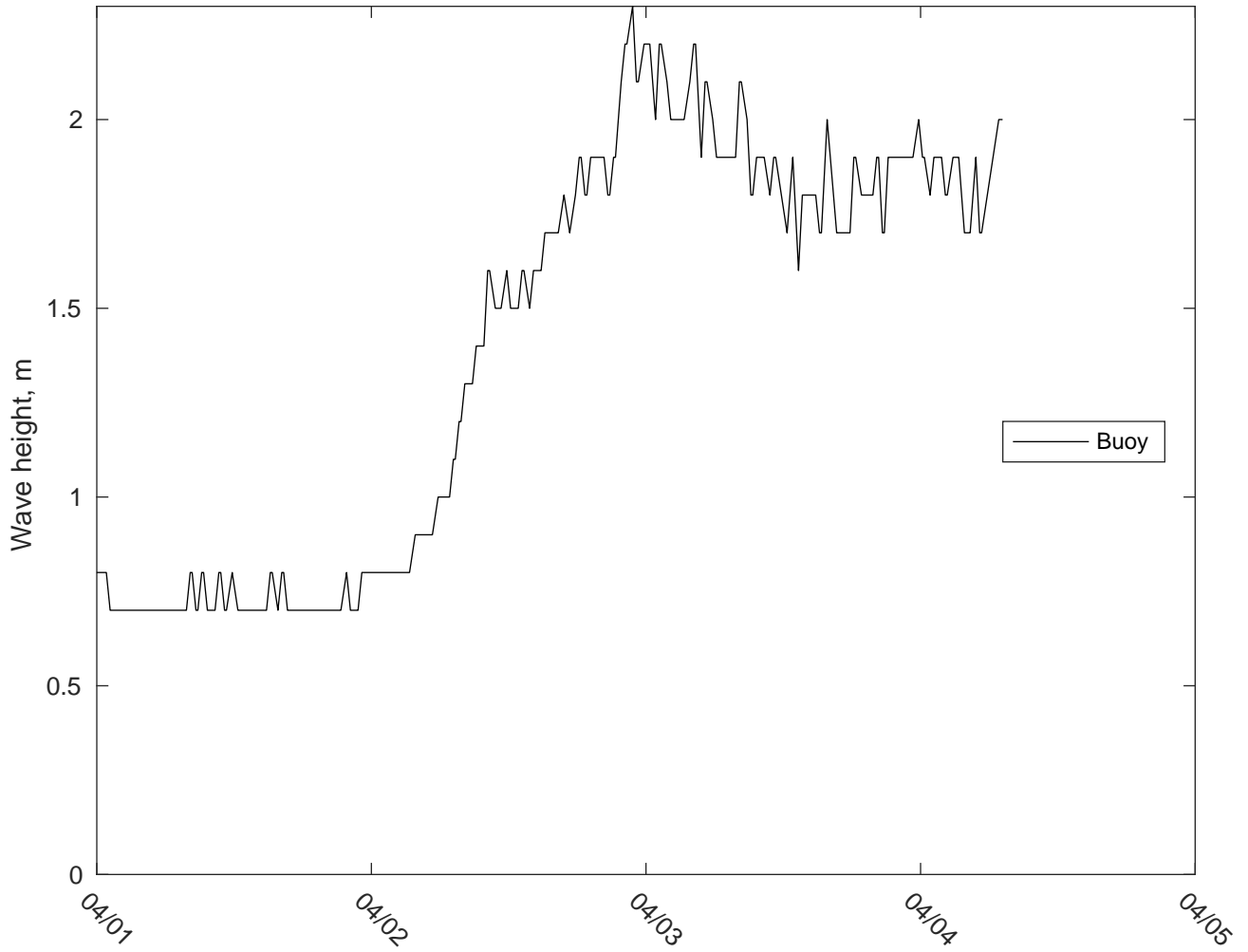
NDBC 42035 vs AUSWAV Waves: 10 to 16 day forecast
