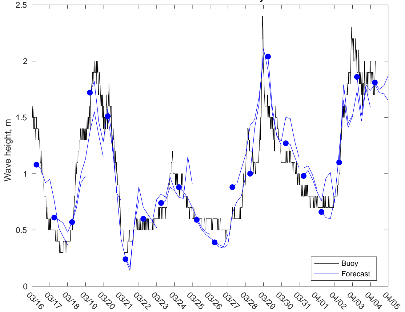
NDBC 42035 vs AUSWAV Waves: 3 to 5 day forecast
