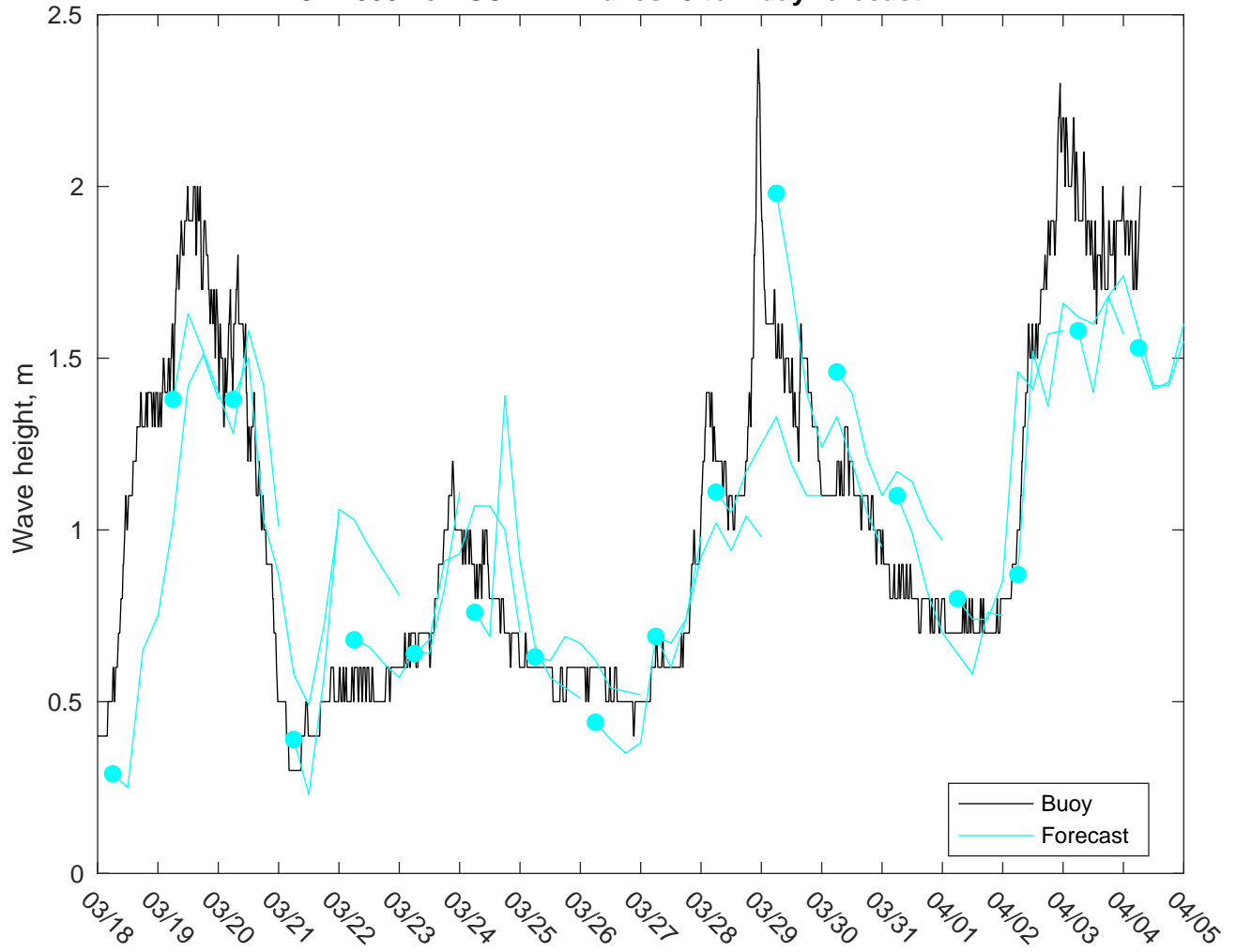
NDBC 42035 vs AUSWAV Waves: 5 to 7 day forecast
