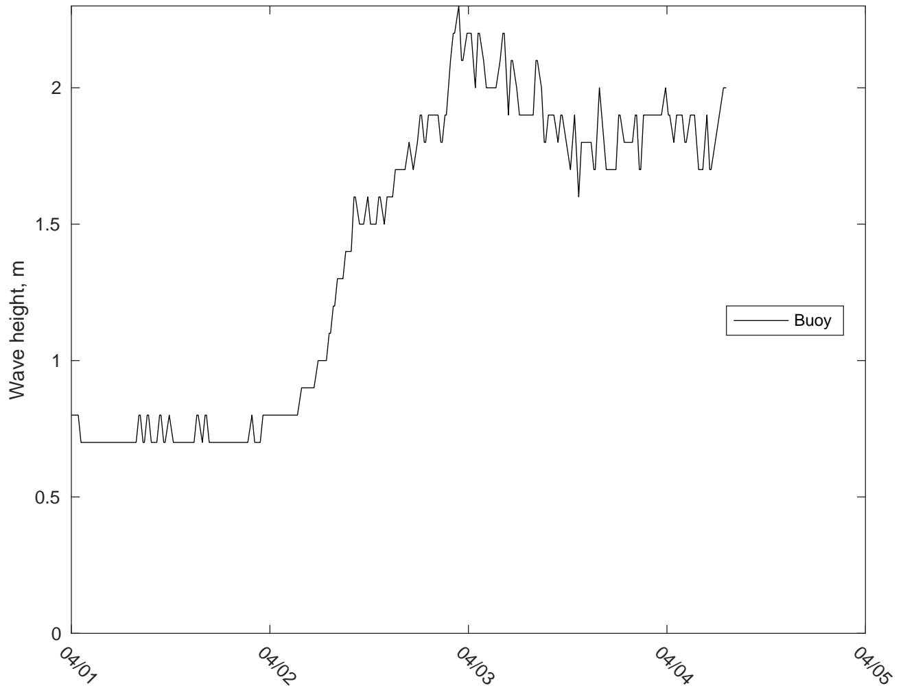
NDBC 42035 vs AUSWAV Waves: 7 to 10 day forecast
