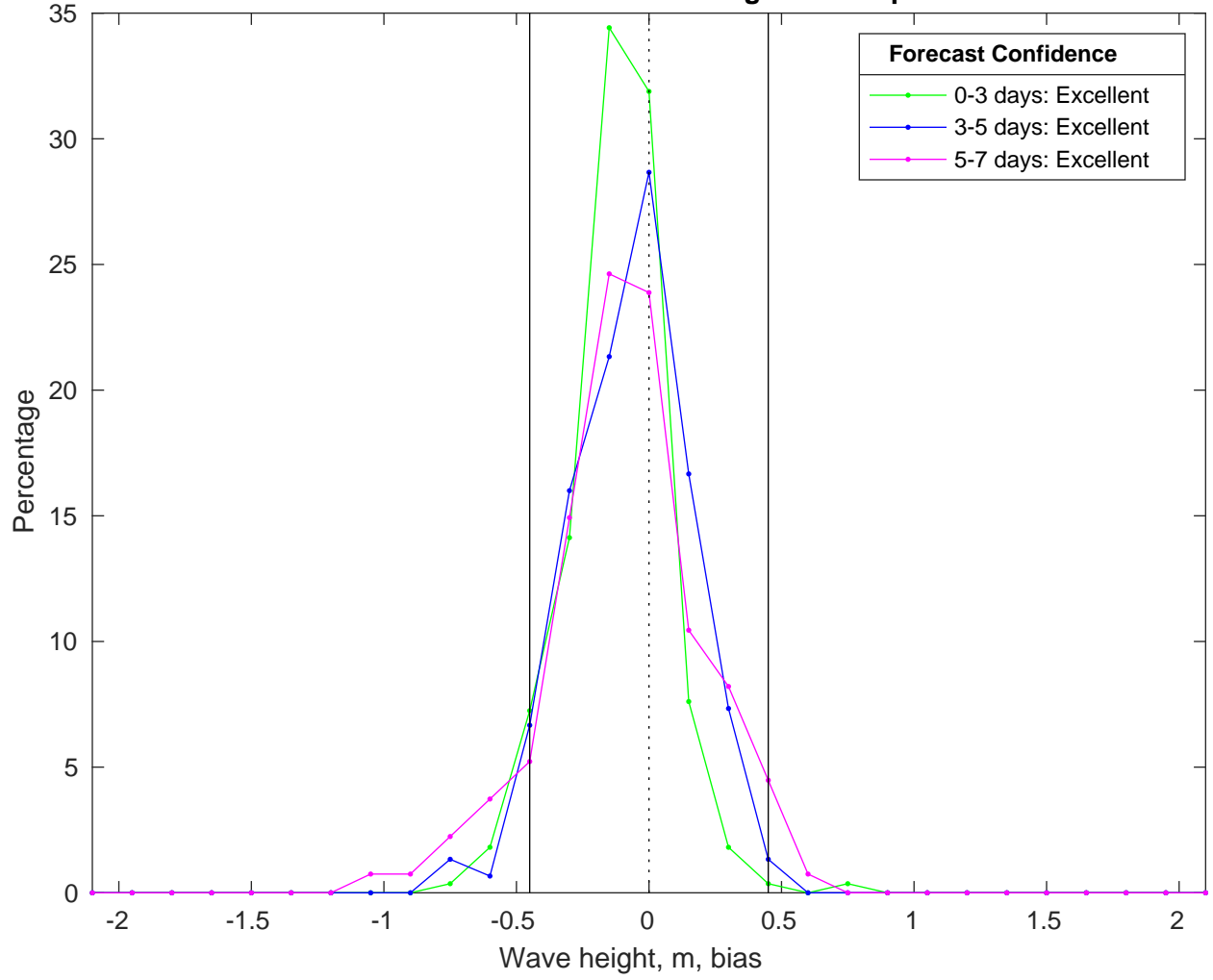
NDBC 42035 vs AUSWAV Waves Bias Histogram: 04-Apr-2025
