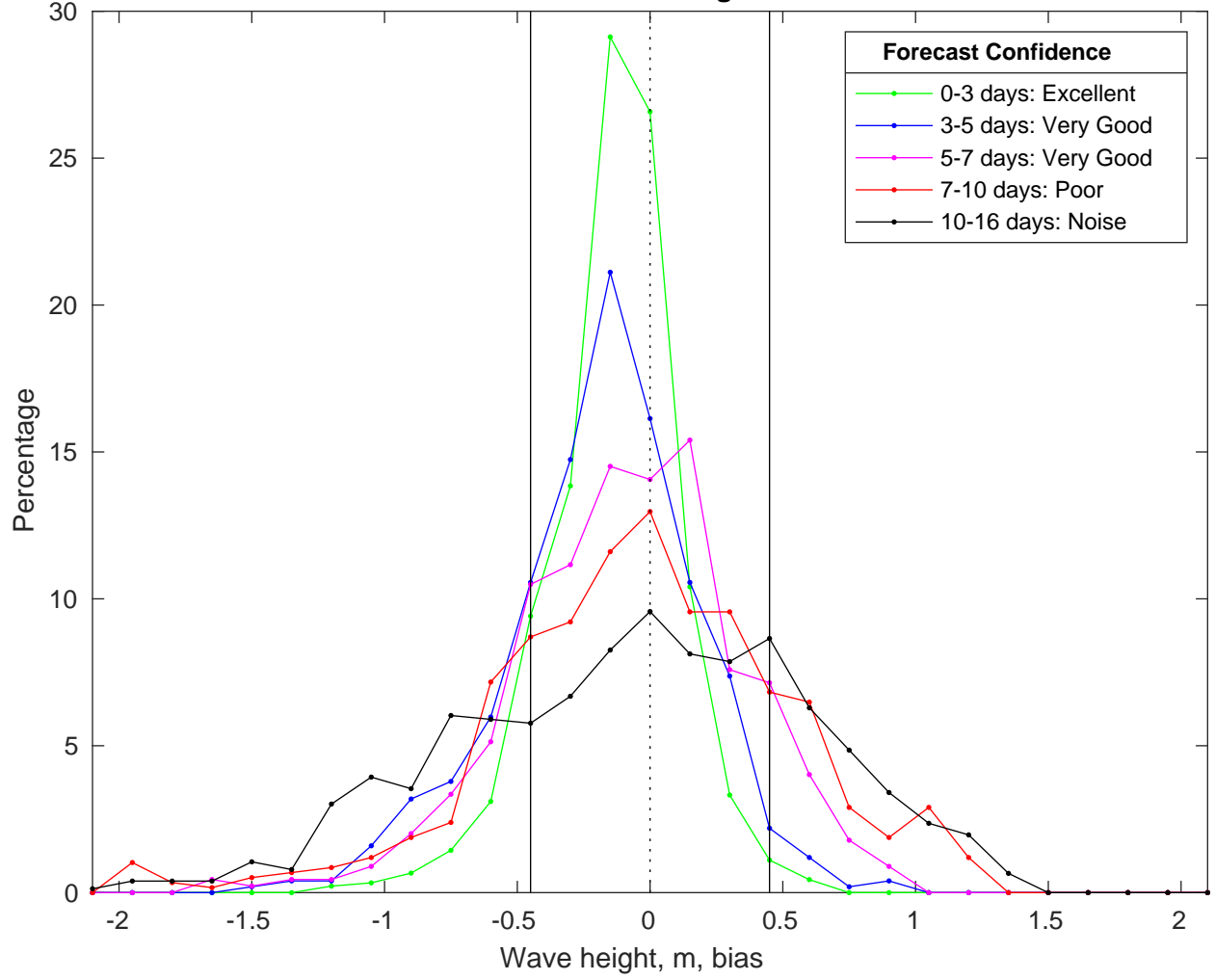
NDBC 42035 vs GFSWaves Bias Histogram: 18-Jan-2025
